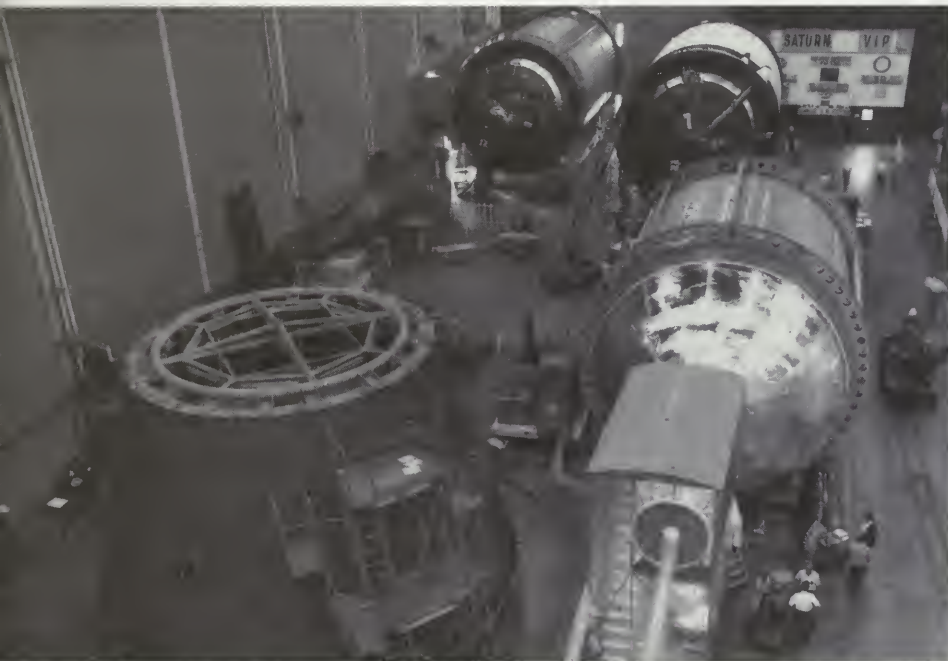
NASA's Manned Flight Awareness program made its mark in all major contractor operations (see diagram). This scene is in the Douglas plant; S-IVB stages are being fabricated and assembled under the banner on the far wall, "Saturn VIP," which in Douglas stood for their "Very Important People" who had made safety or quality assurance contributions.
