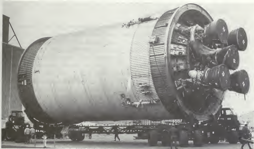
An S-II stage on its transporter.
