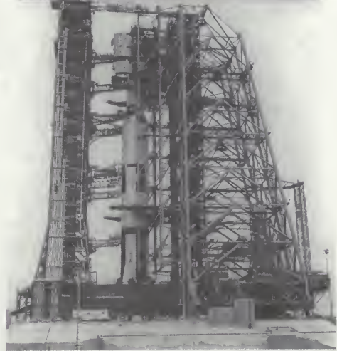
MOBILE SERVICE STRUCTURES ON PAD 39A WITH SATURN V ON MOBILE LAUNCHER-KSC
